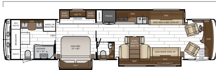
Length: 43' 09"
