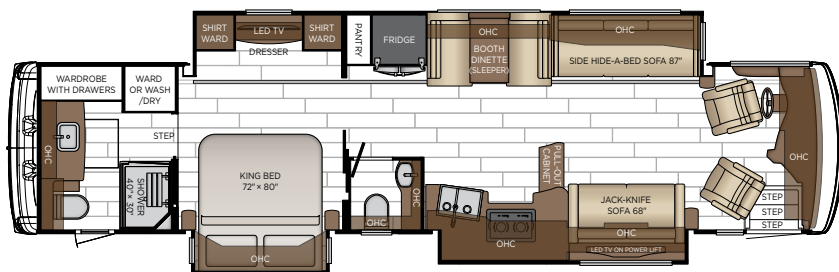
Length: 40' 09"
