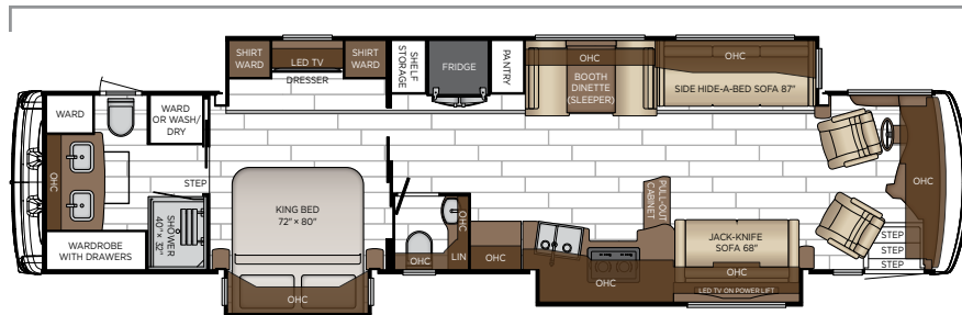
Length: 43' 09"
