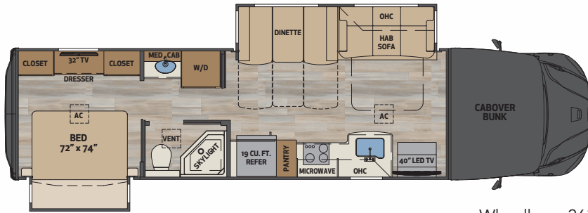
Wheelbase 263"
