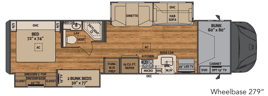
38BB 38' mid bath, 2 slides
