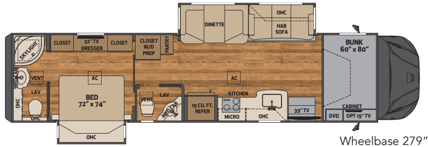
38RB 38' mid and rear bath, 2 slides
